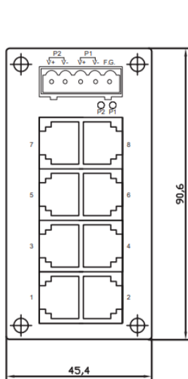
Front-panel front view
